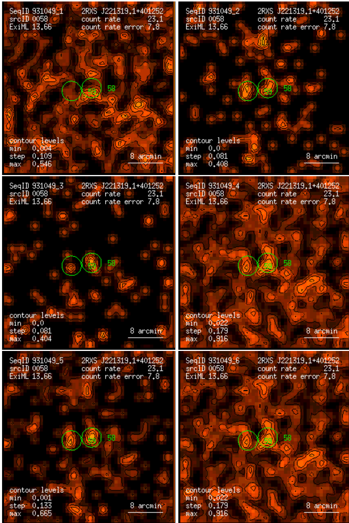
Figure 58: RASS 931049: detection 0058: band rate images, Gaussian filter: (1) PSPC channels 11 – 41, (2) 52 – 90, (3) 91 – 201, (4) 11 – 235, (5) 52 – 201, (6) 11 – 201. Broad band rates in counts/ks. Band rate contour levels in counts/ks/arcmin 2 .
