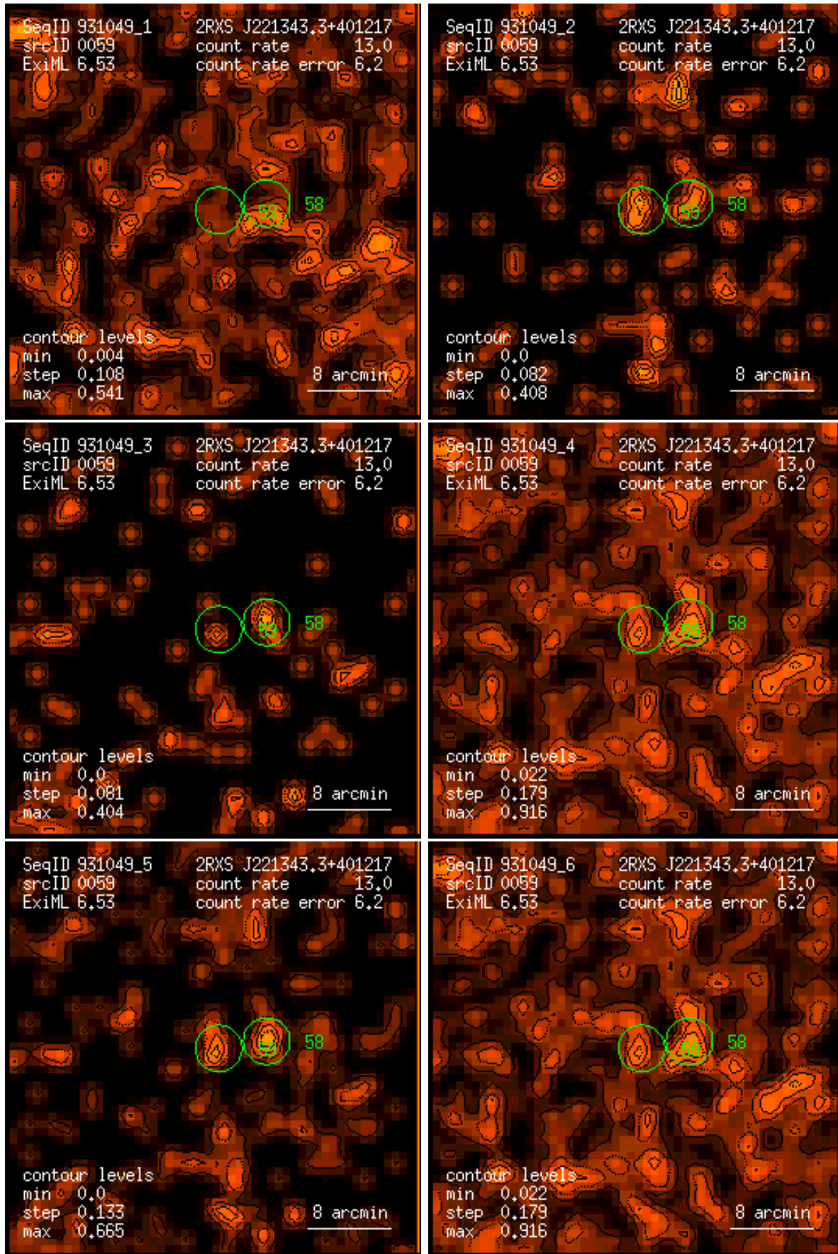
Figure 59: RASS 931049: detection 0059: band rate images, Gaussian filter: (1) PSPC channels 11 – 41, (2) 52 – 90, (3) 91 – 201, (4) 11 – 235, (5) 52 – 201, (6) 11 – 201. Broad band rates in counts/ks. Band rate contour levels in counts/ks/arcmin 2 .
