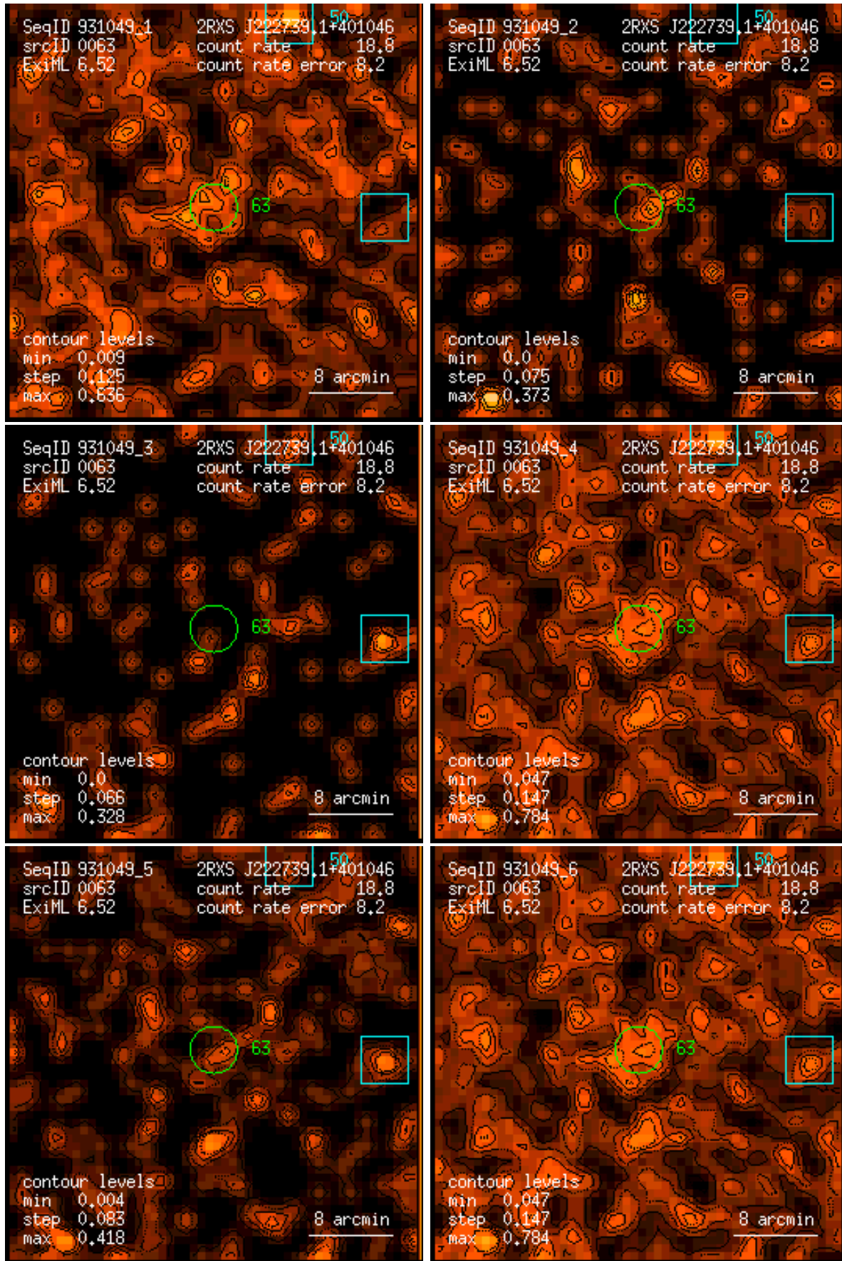
Figure 63: RASS 931049: detection 0063: band rate images, Gaussian filter: (1) PSPC channels 11 – 41, (2) 52 – 90, (3) 91 – 201, (4) 11 – 235, (5) 52 – 201, (6) 11 – 201. Broad band rates in counts/ks. Band rate contour levels in counts/ks/arcmin 2 .
