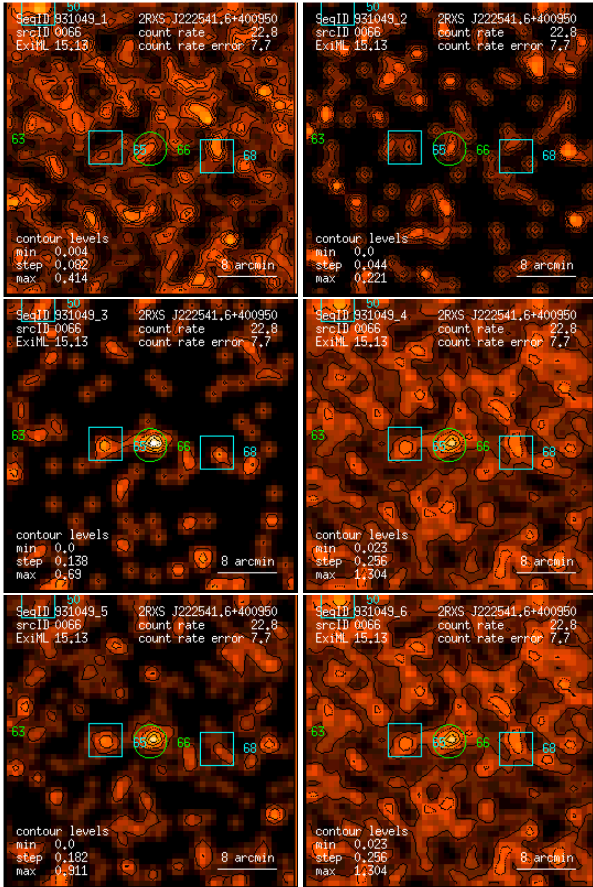
Figure 66: RASS 931049: detection 0066: band rate images, Gaussian filter: (1) PSPC channels 11 – 41, (2) 52 – 90, (3) 91 – 201, (4) 11 – 235, (5) 52 – 201, (6) 11 – 201. Broad band rates in counts/ks. Band rate contour levels in counts/ks/arcmin 2 .
