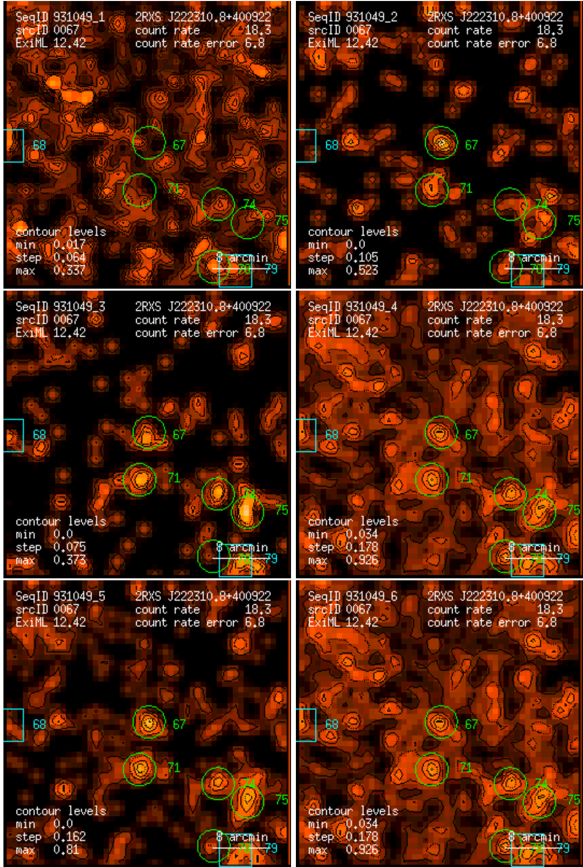
Figure 67: RASS 931049: detection 0067: band rate images, Gaussian filter: (1) PSPC channels 11 – 41, (2) 52 – 90, (3) 91 – 201, (4) 11 – 235, (5) 52 – 201, (6) 11 – 201. Broad band rates in counts/ks. Band rate contour levels in counts/ks/arcmin 2 .
