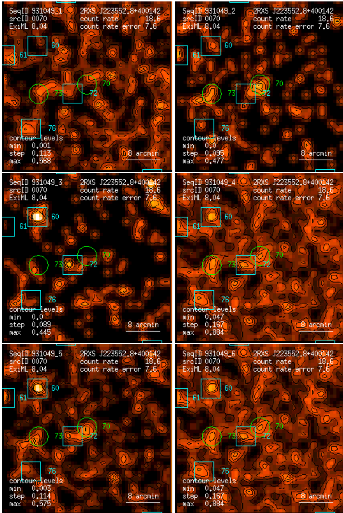
Figure 70: RASS 931049: detection 0070: band rate images, Gaussian filter: (1) PSPC channels 11 – 41, (2) 52 – 90, (3) 91 – 201, (4) 11 – 235, (5) 52 – 201, (6) 11 – 201. Broad band rates in counts/ks. Band rate contour levels in counts/ks/arcmin 2 .
