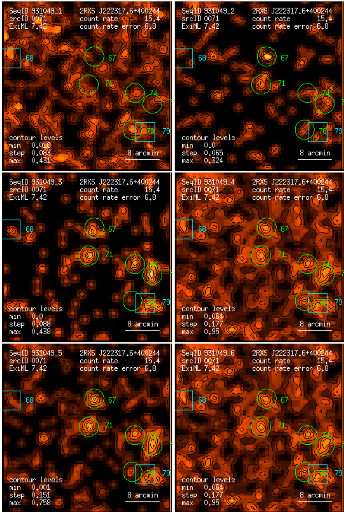
Figure 71: RASS 931049: detection 0071: band rate images, Gaussian filter: (1) PSPC channels 11 – 41, (2) 52 – 90, (3) 91 – 201, (4) 11 – 235, (5) 52 – 201, (6) 11 – 201. Broad band rates in counts/ks. Band rate contour levels in counts/ks/arcmin 2 .
