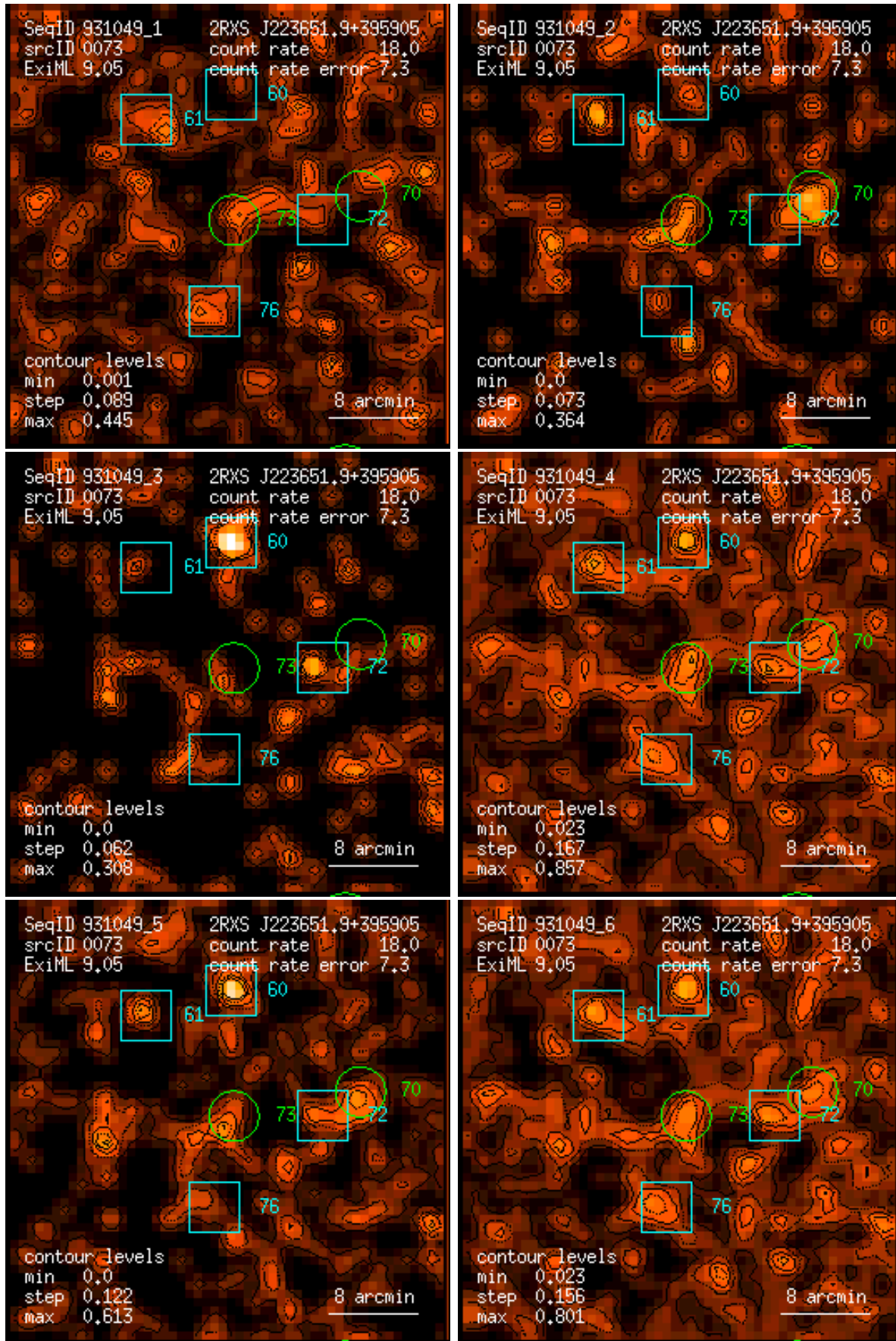
Figure 73: RASS 931049: detection 0073: band rate images, Gaussian filter: (1) PSPC channels 11 – 41, (2) 52 – 90, (3) 91 – 201, (4) 11 – 235, (5) 52 – 201, (6) 11 – 201. Broad band rates in counts/ks. Band rate contour levels in counts/ks/arcmin 2 .
