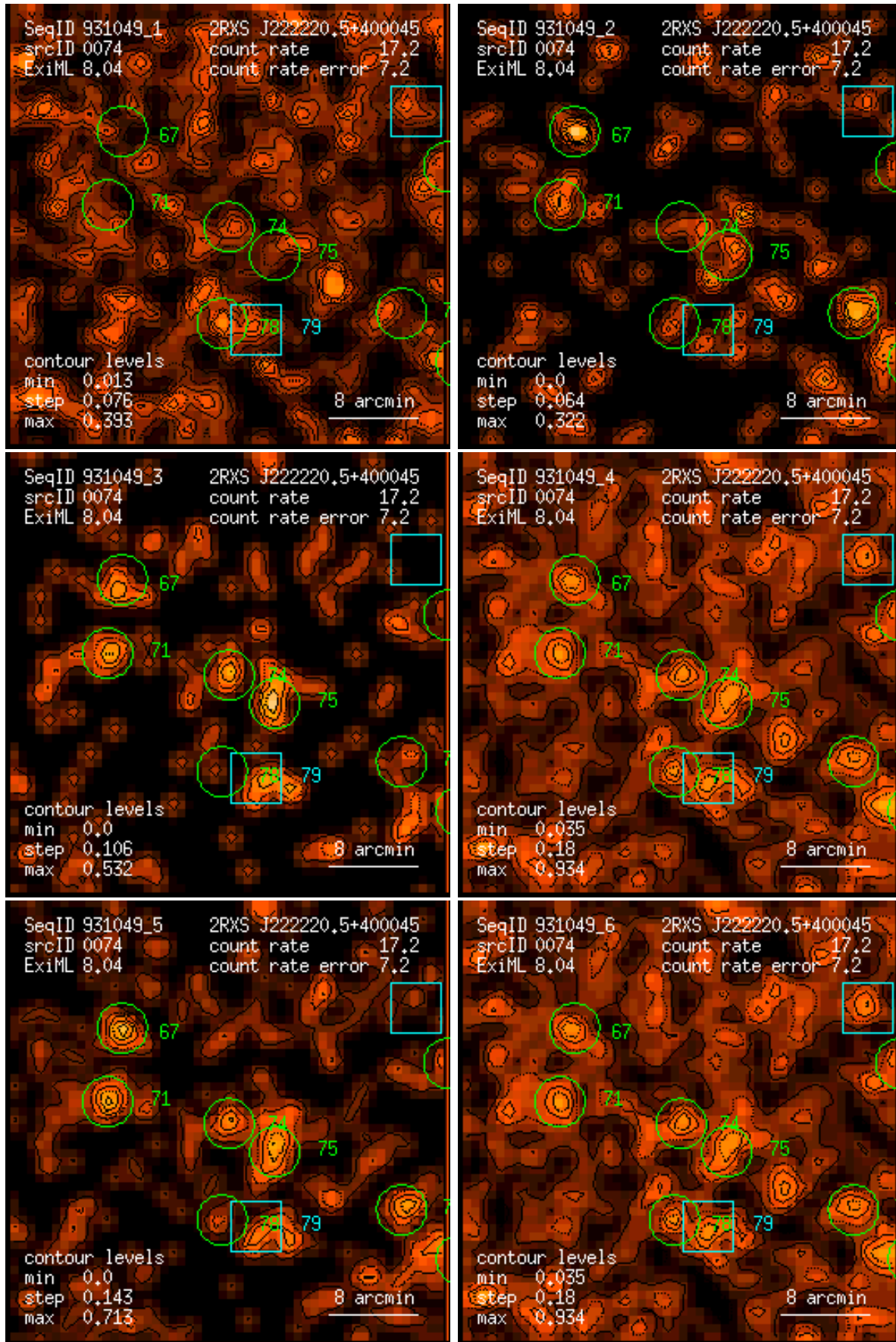
Figure 74: RASS 931049: detection 0074: band rate images, Gaussian filter: (1) PSPC channels 11 – 41, (2) 52 – 90, (3) 91 – 201, (4) 11 – 235, (5) 52 – 201, (6) 11 – 201. Broad band rates in counts/ks. Band rate contour levels in counts/ks/arcmin 2 .
