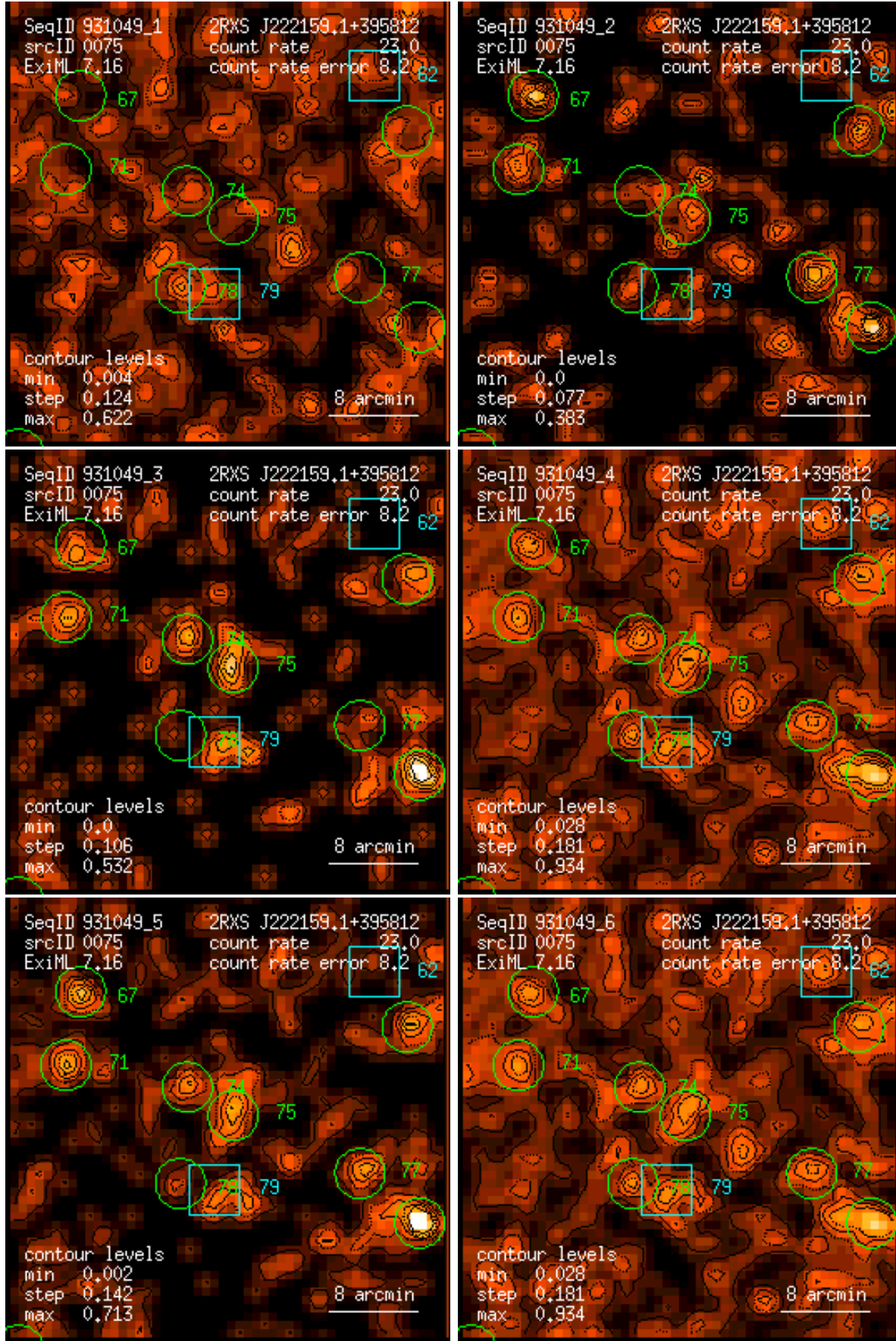
Figure 75: RASS 931049: detection 0075: band rate images, Gaussian filter: (1) PSPC channels 11 – 41, (2) 52 – 90, (3) 91 – 201, (4) 11 – 235, (5) 52 – 201, (6) 11 – 201. Broad band rates in counts/ks. Band rate contour levels in counts/ks/arcmin 2 .
