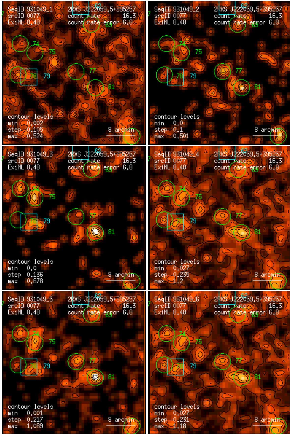
Figure 77: RASS 931049: detection 0077: band rate images, Gaussian filter: (1) PSPC channels 11 – 41, (2) 52 – 90, (3) 91 – 201, (4) 11 – 235, (5) 52 – 201, (6) 11 – 201. Broad band rates in counts/ks. Band rate contour levels in counts/ks/arcmin 2 .
