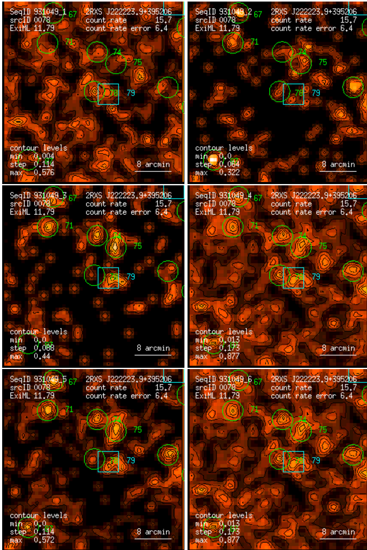
Figure 78: RASS 931049: detection 0078: band rate images, Gaussian filter: (1) PSPC channels 11 – 41, (2) 52 – 90, (3) 91 – 201, (4) 11 – 235, (5) 52 – 201, (6) 11 – 201. Broad band rates in counts/ks. Band rate contour levels in counts/ks/arcmin 2 .
