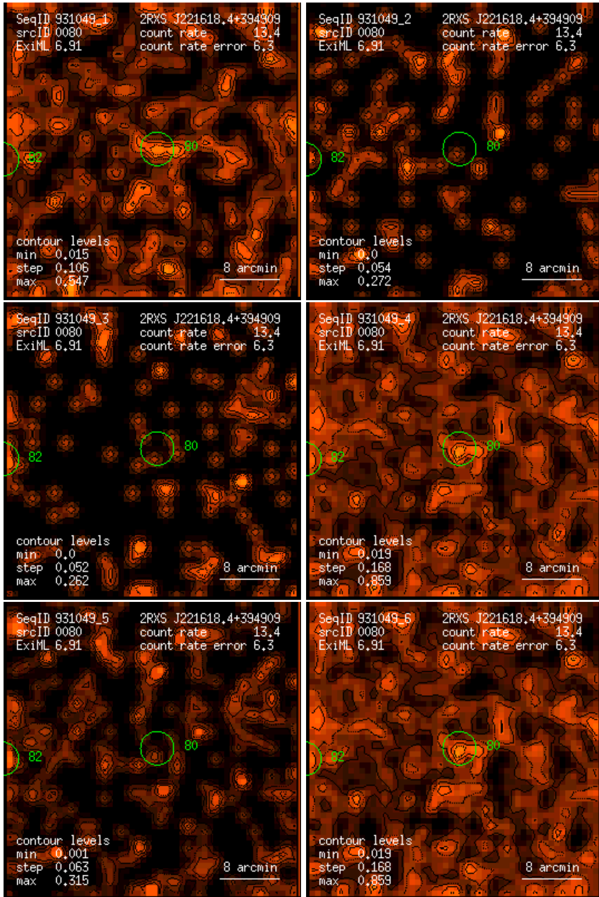
Figure 80: RASS 931049: detection 0080: band rate images, Gaussian filter: (1) PSPC channels 11 – 41, (2) 52 – 90, (3) 91 – 201, (4) 11 – 235, (5) 52 – 201, (6) 11 – 201. Broad band rates in counts/ks. Band rate contour levels in counts/ks/arcmin 2 .
