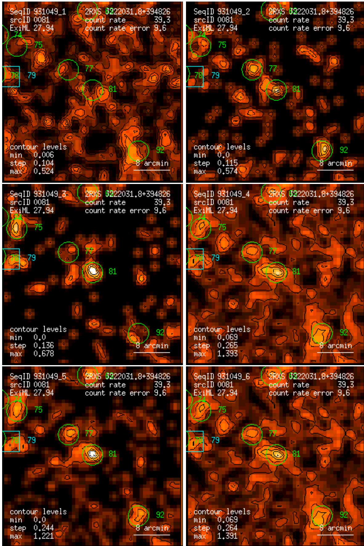
Figure 81: RASS 931049: detection 0081: band rate images, Gaussian filter: (1) PSPC channels 11 – 41, (2) 52 – 90, (3) 91 – 201, (4) 11 – 235, (5) 52 – 201, (6) 11 – 201. Broad band rates in counts/ks. Band rate contour levels in counts/ks/arcmin 2 .
