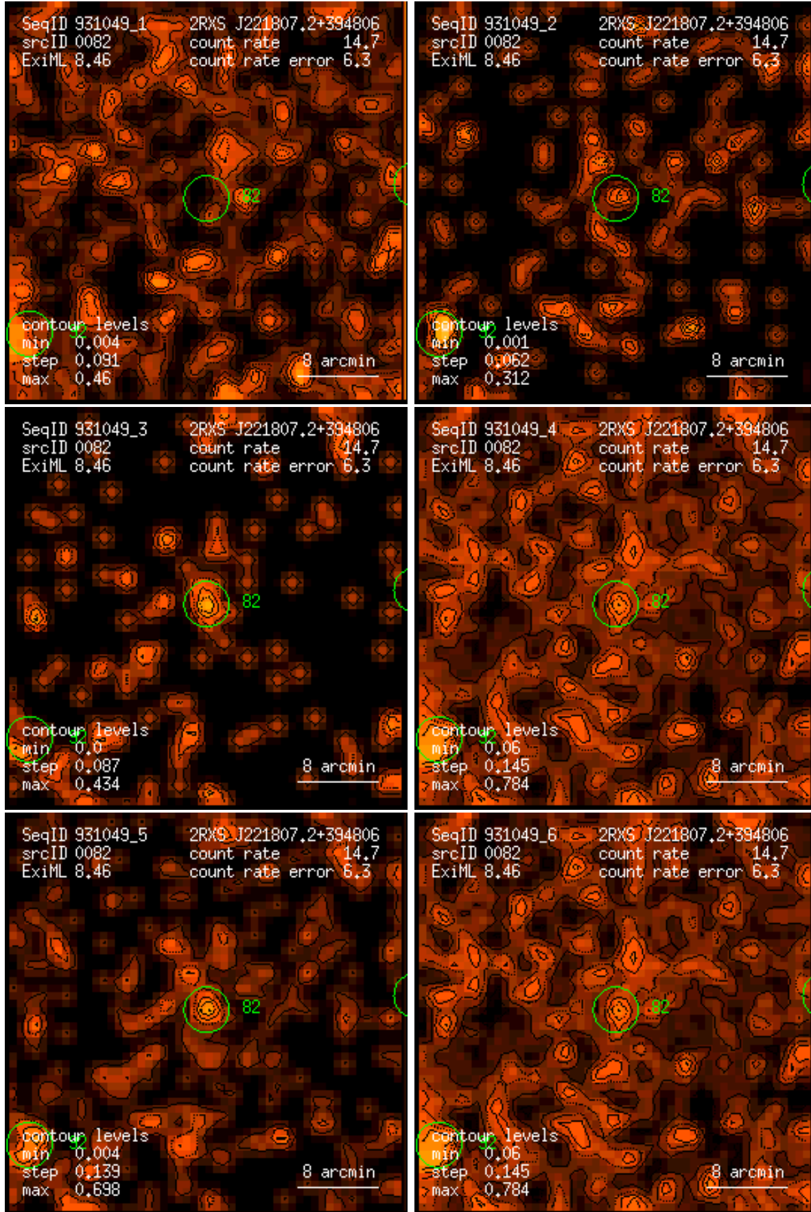
Figure 82: RASS 931049: detection 0082: band rate images, Gaussian filter: (1) PSPC channels 11 – 41, (2) 52 – 90, (3) 91 – 201, (4) 11 – 235, (5) 52 – 201, (6) 11 – 201. Broad band rates in counts/ks. Band rate contour levels in counts/ks/arcmin 2 .
