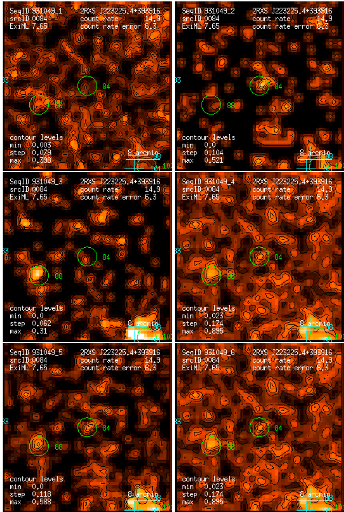
Figure 84: RASS 931049: detection 0084: band rate images, Gaussian filter: (1) PSPC channels 11 – 41, (2) 52 – 90, (3) 91 – 201, (4) 11 – 235, (5) 52 – 201, (6) 11 – 201. Broad band rates in counts/ks. Band rate contour levels in counts/ks/arcmin 2 .
