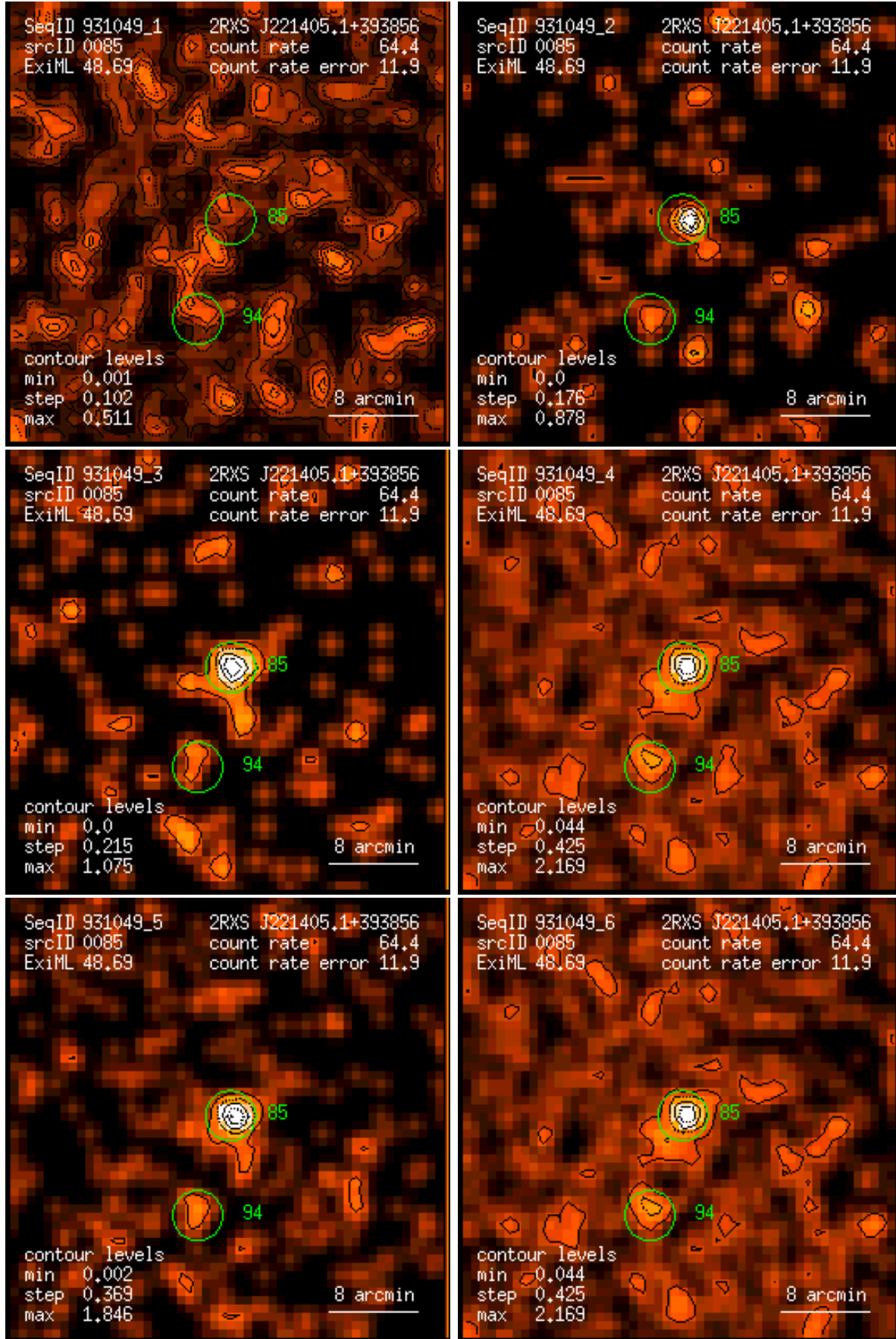
Figure 85: RASS 931049: detection 0085: band rate images, Gaussian filter: (1) PSPC channels 11 – 41, (2) 52 – 90, (3) 91 – 201, (4) 11 – 235, (5) 52 – 201, (6) 11 – 201. Broad band rates in counts/ks. Band rate contour levels in counts/ks/arcmin 2 .
