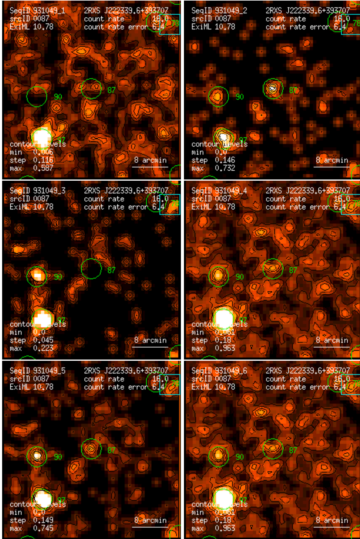
Figure 87: RASS 931049: detection 0087: band rate images, Gaussian filter: (1) PSPC channels 11 – 41, (2) 52 – 90, (3) 91 – 201, (4) 11 – 235, (5) 52 – 201, (6) 11 – 201. Broad band rates in counts/ks. Band rate contour levels in counts/ks/arcmin 2 .
