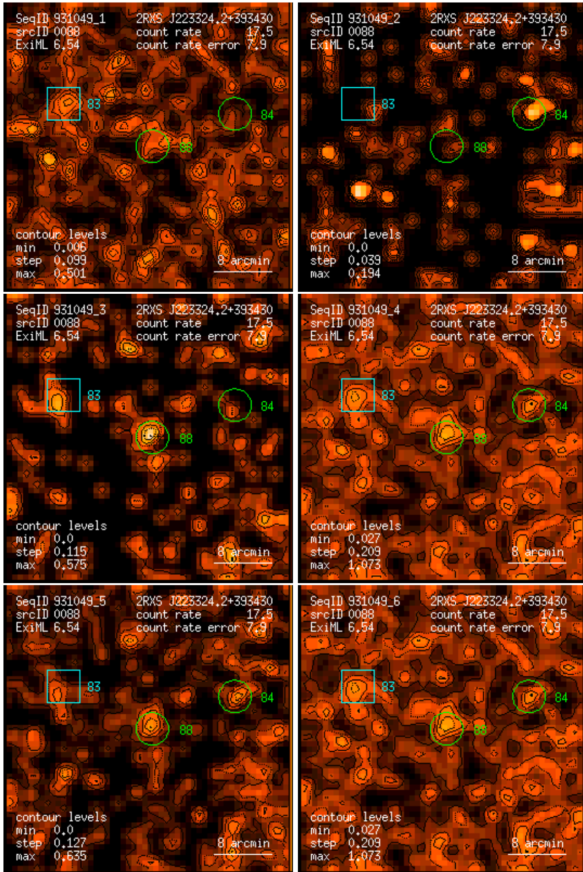
Figure 88: RASS 931049: detection 0088: band rate images, Gaussian filter: (1) PSPC channels 11 – 41, (2) 52 – 90, (3) 91 – 201, (4) 11 – 235, (5) 52 – 201, (6) 11 – 201. Broad band rates in counts/ks. Band rate contour levels in counts/ks/arcmin 2 .
