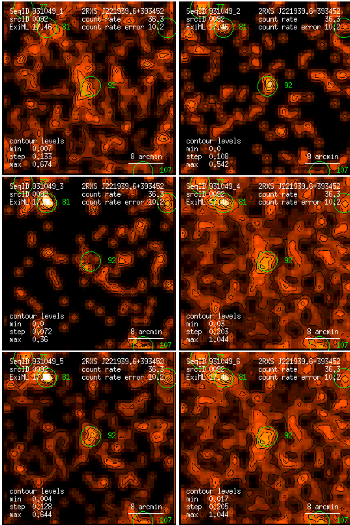
Figure 92: RASS 931049: detection 0092: band rate images, Gaussian filter: (1) PSPC channels 11 – 41, (2) 52 – 90, (3) 91 – 201, (4) 11 – 235, (5) 52 – 201, (6) 11 – 201. Broad band rates in counts/ks. Band rate contour levels in counts/ks/arcmin 2 .
