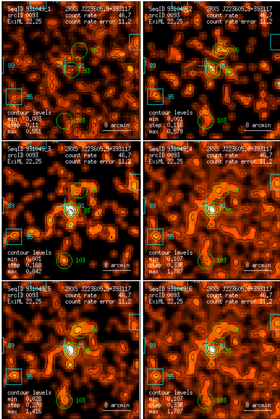
Figure 93: RASS 931049: detection 0093: band rate images, Gaussian filter: (1) PSPC channels 11 – 41, (2) 52 – 90, (3) 91 – 201, (4) 11 – 235, (5) 52 – 201, (6) 11 – 201. Broad band rates in counts/ks. Band rate contour levels in counts/ks/arcmin 2 .
