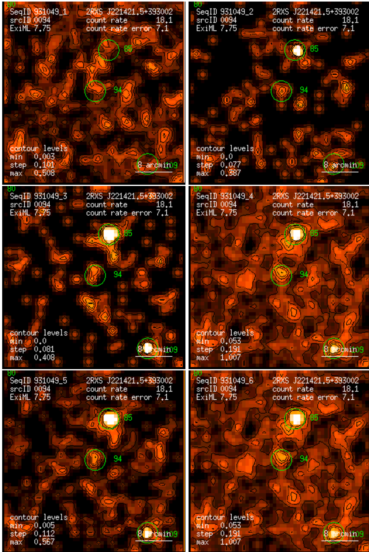
Figure 94: RASS 931049: detection 0094: band rate images, Gaussian filter: (1) PSPC channels 11 – 41, (2) 52 – 90, (3) 91 – 201, (4) 11 – 235, (5) 52 – 201, (6) 11 – 201. Broad band rates in counts/ks. Band rate contour levels in counts/ks/arcmin 2 .
