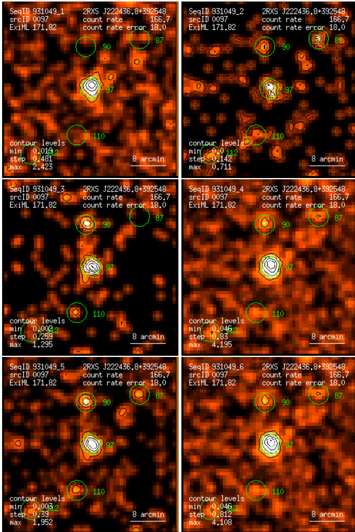
Figure 97: RASS 931049: detection 0097: band rate images, Gaussian filter: (1) PSPC channels 11 – 41, (2) 52 – 90, (3) 91 – 201, (4) 11 – 235, (5) 52 – 201, (6) 11 – 201. Broad band rates in counts/ks. Band rate contour levels in counts/ks/arcmin 2 .
