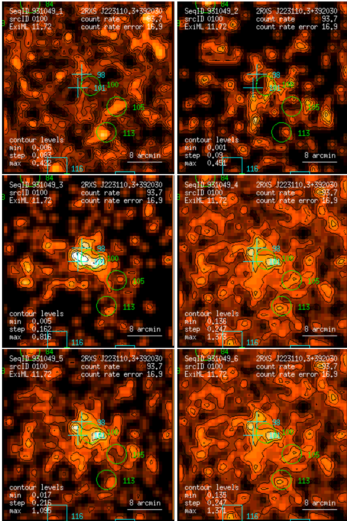
Figure 100: RASS 931049: detection 0100: band rate images, Gaussian filter: (1) PSPC channels 11 – 41, (2) 52 – 90, (3) 91 – 201, (4) 11 – 235, (5) 52 – 201, (6) 11 – 201. Broad band rates in counts/ks. Band rate contour levels in counts/ks/arcmin 2 .
