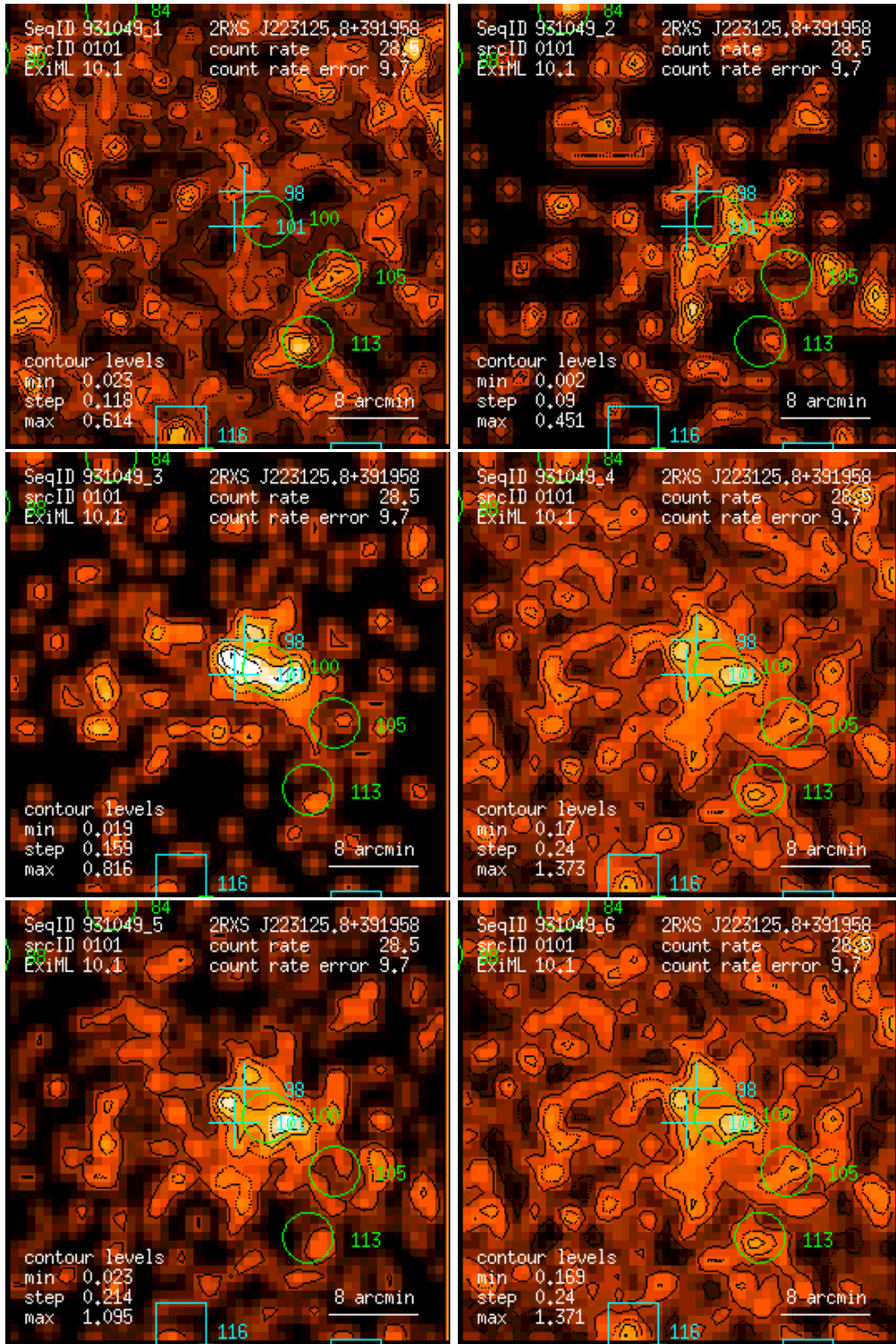
Figure 101: RASS 931049: detection 0101: band rate images, Gaussian filter: (1) PSPC channels 11 – 41, (2) 52 – 90, (3) 91 – 201, (4) 11 – 235, (5) 52 – 201, (6) 11 – 201. Broad band rates in counts/ks. Band rate contour levels in counts/ks/arcmin 2 .
