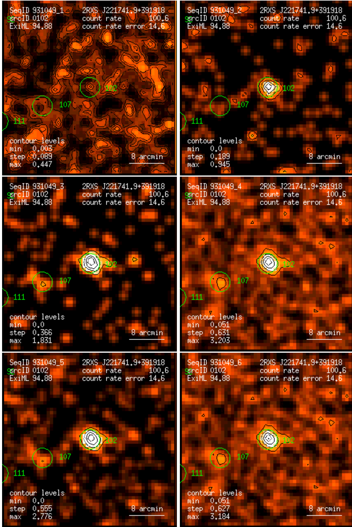
Figure 102: RASS 931049: detection 0102: band rate images, Gaussian filter: (1) PSPC channels 11 – 41, (2) 52 – 90, (3) 91 – 201, (4) 11 – 235, (5) 52 – 201, (6) 11 – 201. Broad band rates in counts/ks. Band rate contour levels in counts/ks/arcmin 2 .
