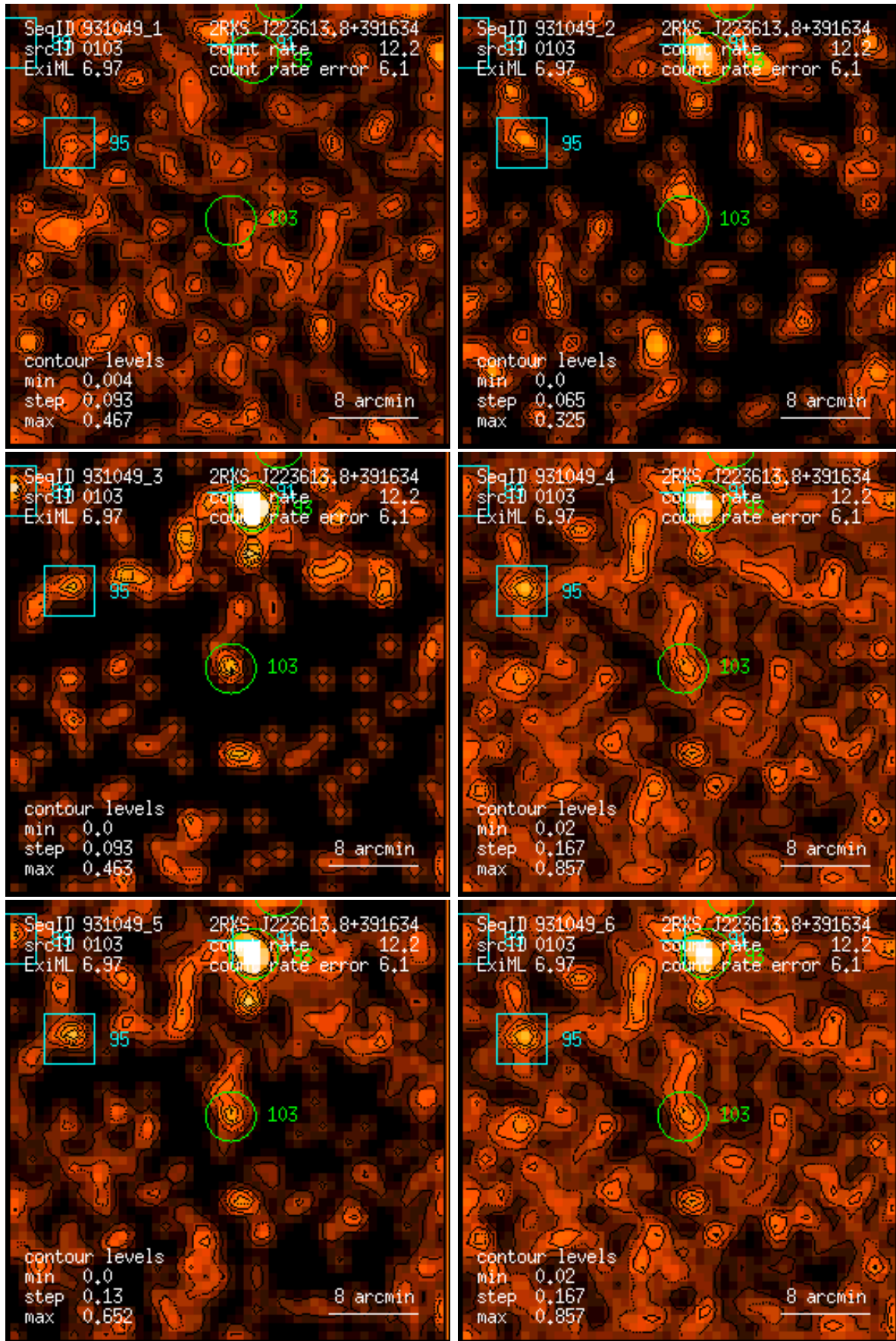
Figure 103: RASS 931049: detection 0103: band rate images, Gaussian filter: (1) PSPC channels 11 – 41, (2) 52 – 90, (3) 91 – 201, (4) 11 – 235, (5) 52 – 201, (6) 11 – 201. Broad band rates in counts/ks. Band rate contour levels in counts/ks/arcmin 2 .
