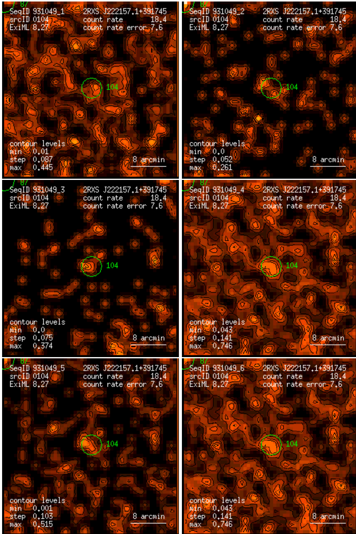
Figure 104: RASS 931049: detection 0104: band rate images, Gaussian filter: (1) PSPC channels 11 – 41, (2) 52 – 90, (3) 91 – 201, (4) 11 – 235, (5) 52 – 201, (6) 11 – 201. Broad band rates in counts/ks. Band rate contour levels in counts/ks/arcmin 2 .
