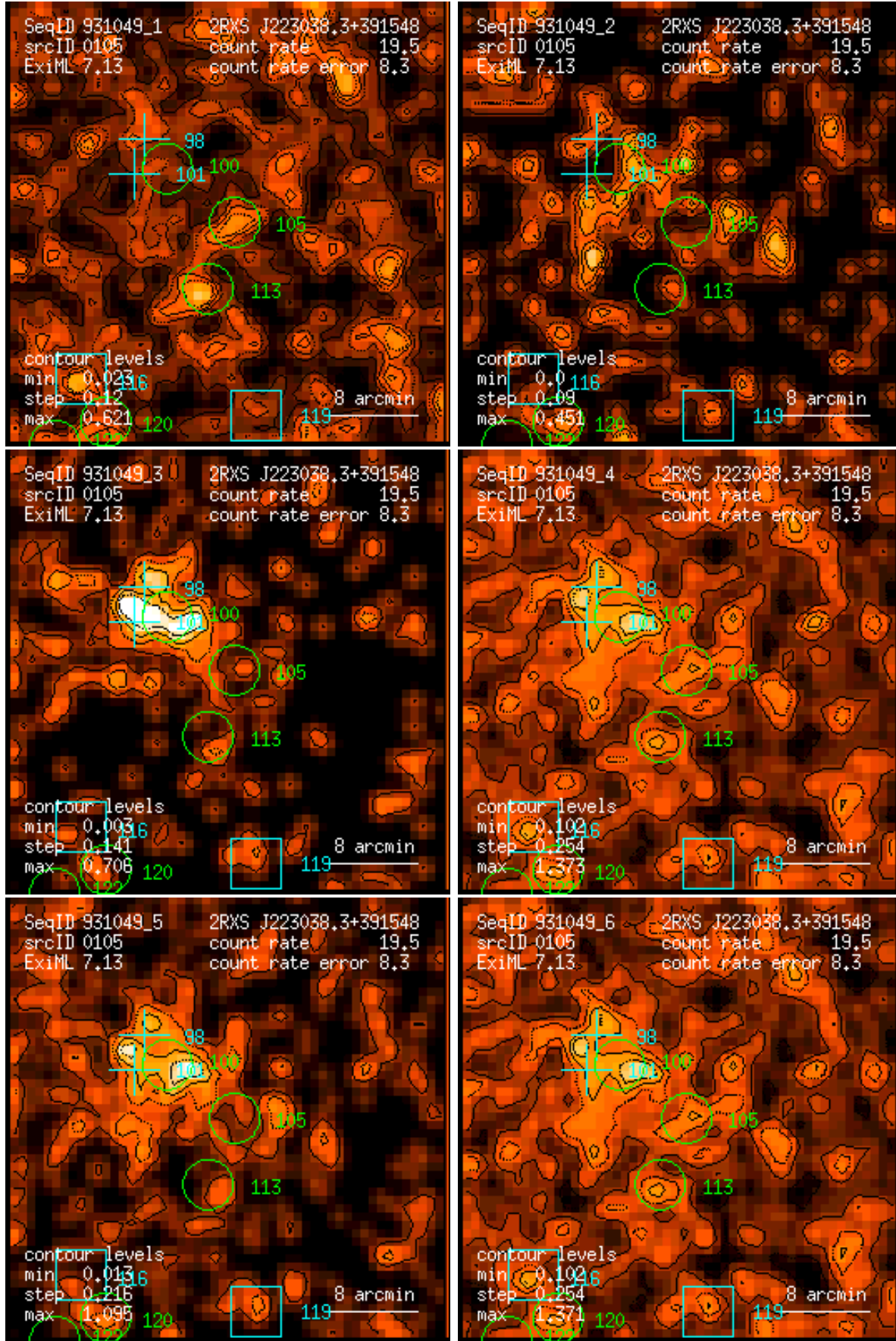
Figure 105: RASS 931049: detection 0105: band rate images, Gaussian filter: (1) PSPC channels 11 – 41, (2) 52 – 90, (3) 91 – 201, (4) 11 – 235, (5) 52 – 201, (6) 11 – 201. Broad band rates in counts/ks. Band rate contour levels in counts/ks/arcmin 2 .
