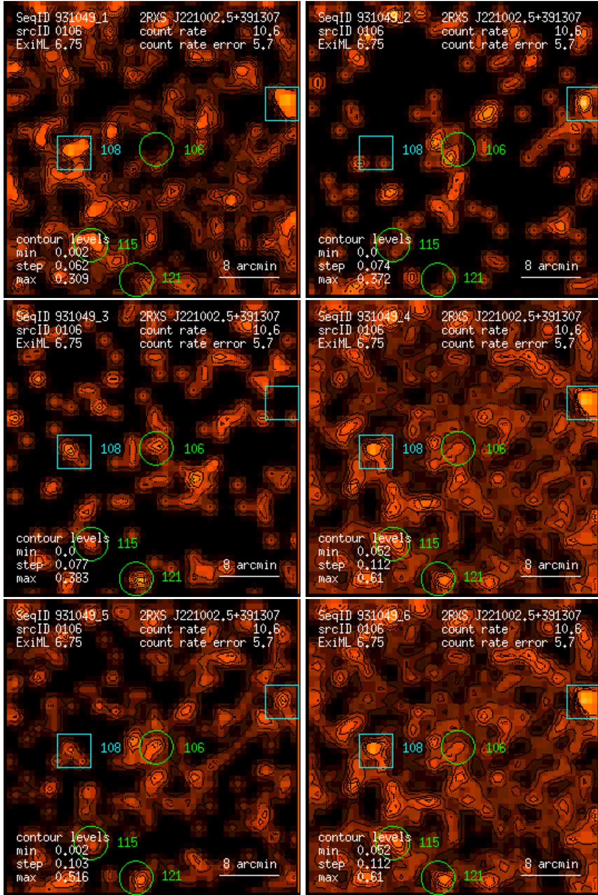
Figure 106: RASS 931049: detection 0106: band rate images, Gaussian filter: (1) PSPC channels 11 – 41, (2) 52 – 90, (3) 91 – 201, (4) 11 – 235, (5) 52 – 201, (6) 11 – 201. Broad band rates in counts/ks. Band rate contour levels in counts/ks/arcmin 2 .
