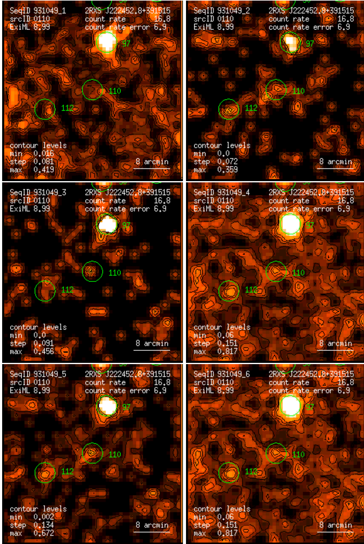
Figure 110: RASS 931049: detection 0110: band rate images, Gaussian filter: (1) PSPC channels 11 – 41, (2) 52 – 90, (3) 91 – 201, (4) 11 – 235, (5) 52 – 201, (6) 11 – 201. Broad band rates in counts/ks. Band rate contour levels in counts/ks/arcmin 2 .
