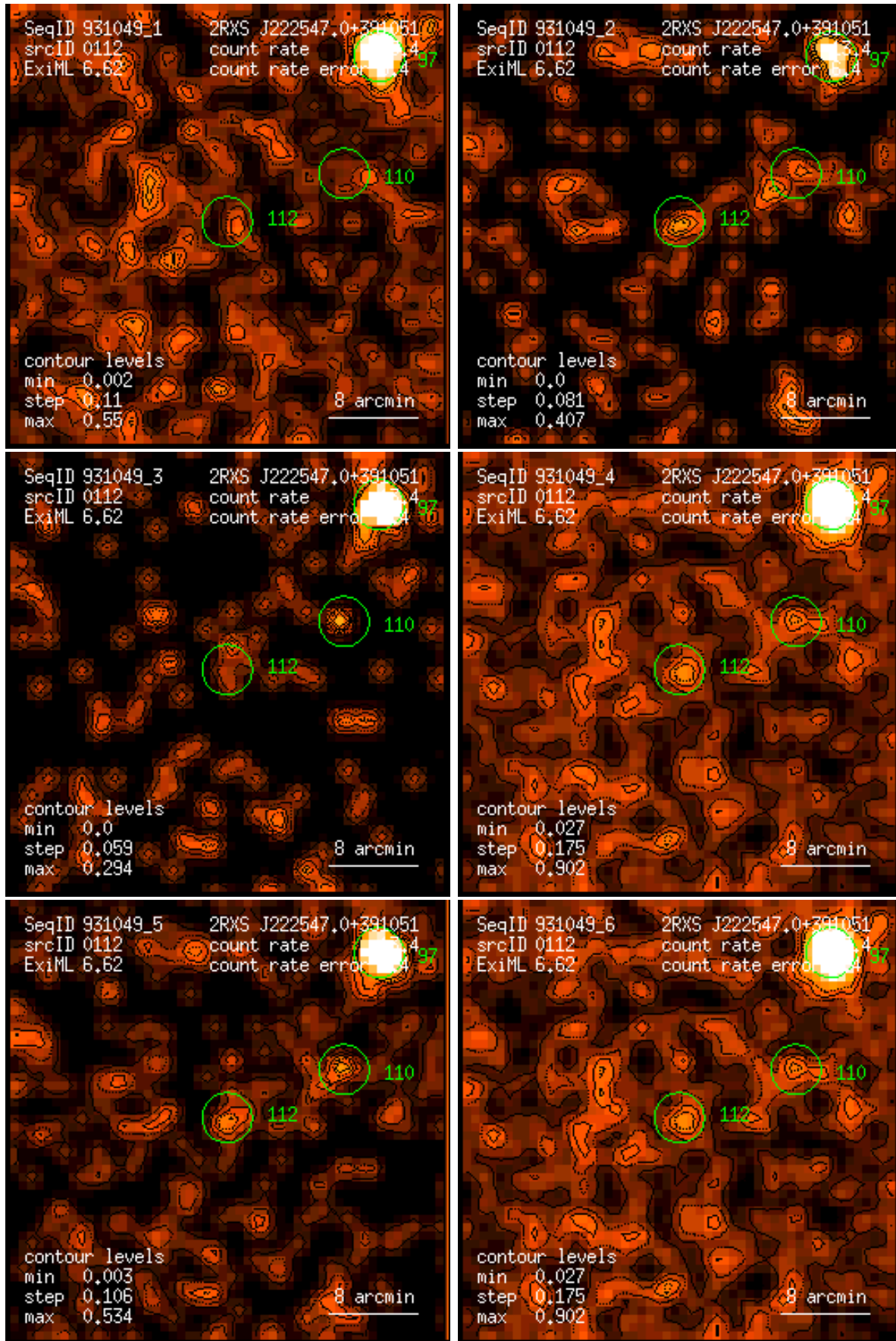
Figure 112: RASS 931049: detection 0112: band rate images, Gaussian filter: (1) PSPC channels 11 – 41, (2) 52 – 90, (3) 91 – 201, (4) 11 – 235, (5) 52 – 201, (6) 11 – 201. Broad band rates in counts/ks. Band rate contour levels in counts/ks/arcmin 2 .
