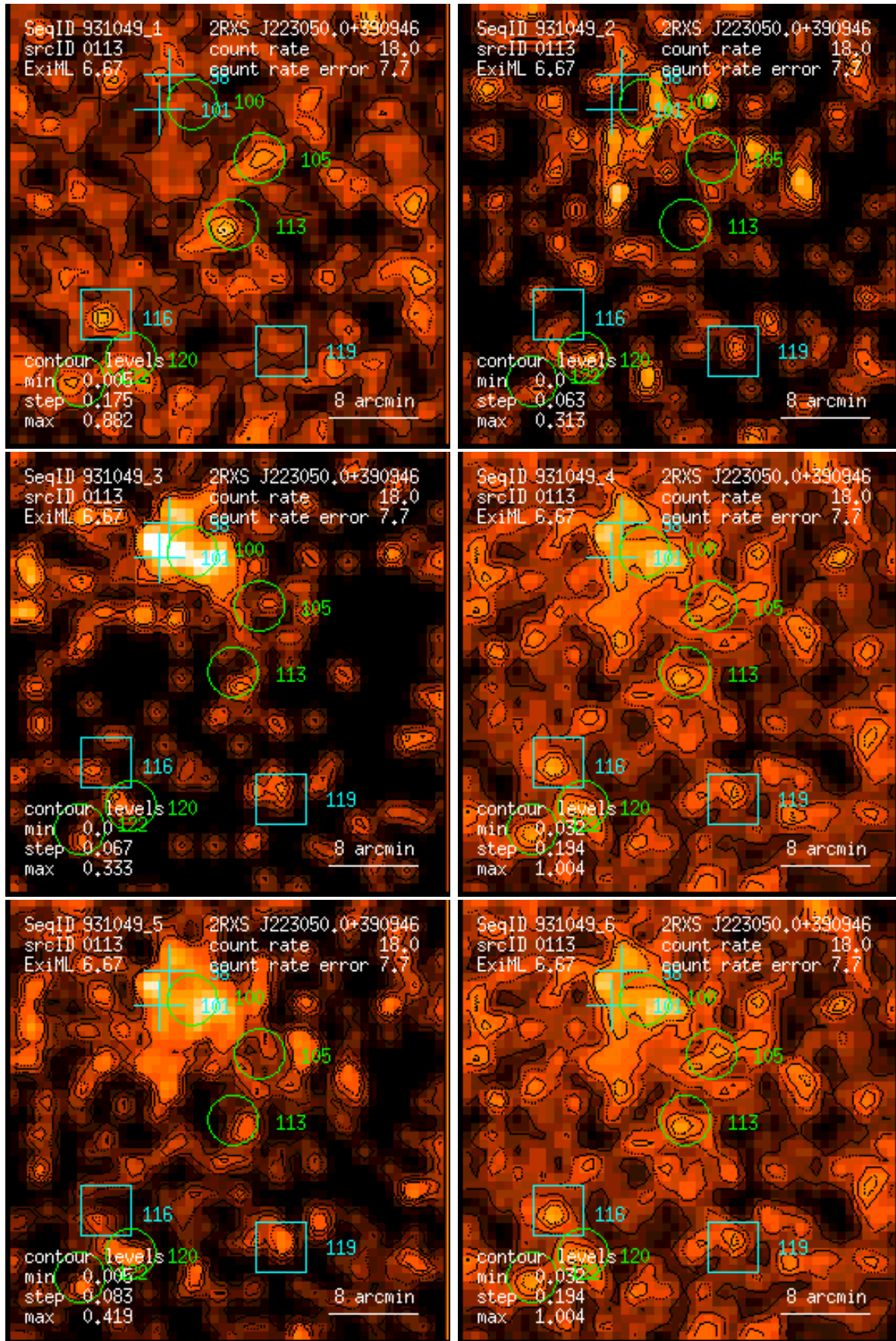
Figure 113: RASS 931049: detection 0113: band rate images, Gaussian filter: (1) PSPC channels 11 – 41, (2) 52 – 90, (3) 91 – 201, (4) 11 – 235, (5) 52 – 201, (6) 11 – 201. Broad band rates in counts/ks. Band rate contour levels in counts/ks/arcmin 2 .
