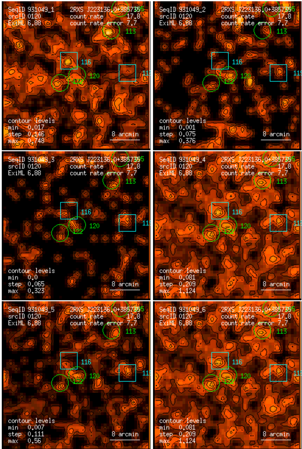
Figure 120: RASS 931049: detection 0120: band rate images, Gaussian filter: (1) PSPC channels 11 – 41, (2) 52 – 90, (3) 91 – 201, (4) 11 – 235, (5) 52 – 201, (6) 11 – 201. Broad band rates in counts/ks. Band rate contour levels in counts/ks/arcmin 2 .
