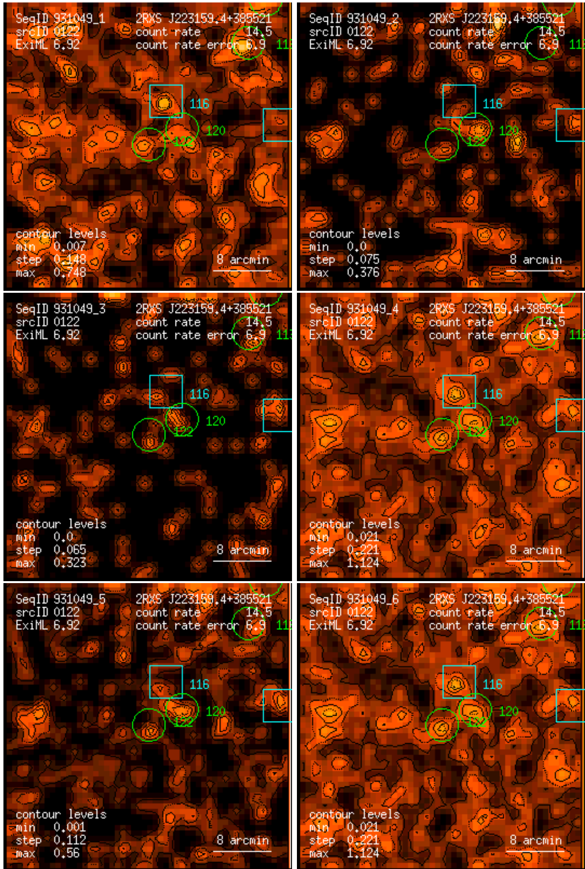
Figure 122: RASS 931049: detection 0122: band rate images, Gaussian filter: (1) PSPC channels 11 – 41, (2) 52 – 90, (3) 91 – 201, (4) 11 – 235, (5) 52 – 201, (6) 11 – 201. Broad band rates in counts/ks. Band rate contour levels in counts/ks/arcmin 2 .
