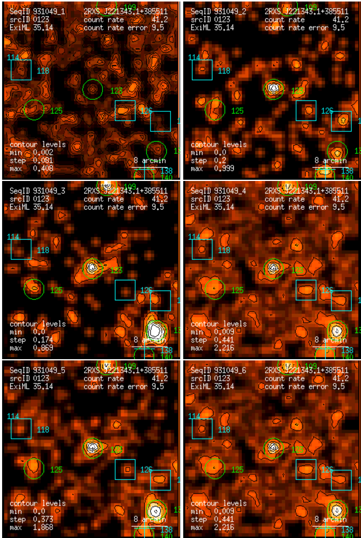
Figure 123: RASS 931049: detection 0123: band rate images, Gaussian filter: (1) PSPC channels 11 – 41, (2) 52 – 90, (3) 91 – 201, (4) 11 – 235, (5) 52 – 201, (6) 11 – 201. Broad band rates in counts/ks. Band rate contour levels in counts/ks/arcmin 2 .
