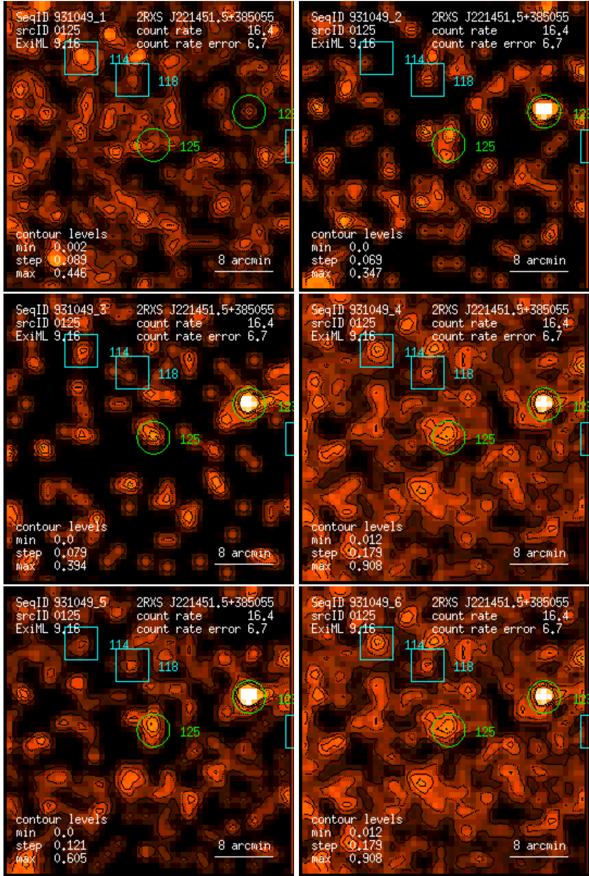
Figure 125: RASS 931049: detection 0125: band rate images, Gaussian filter: (1) PSPC channels 11 – 41, (2) 52 – 90, (3) 91 – 201, (4) 11 – 235, (5) 52 – 201, (6) 11 – 201. Broad band rates in counts/ks. Band rate contour levels in counts/ks/arcmin 2 .
