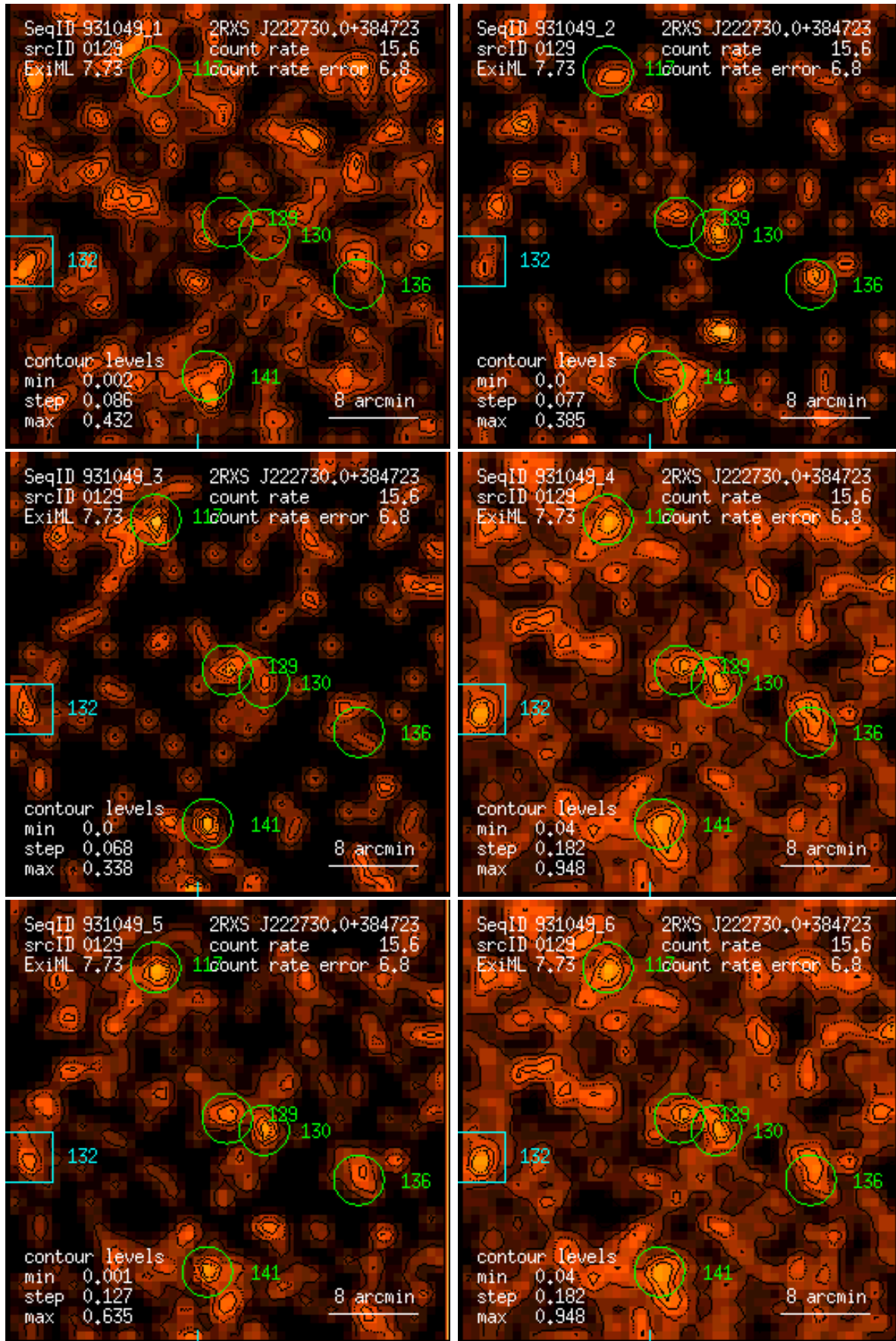
Figure 129: RASS 931049: detection 0129: band rate images, Gaussian filter: (1) PSPC channels 11 – 41, (2) 52 – 90, (3) 91 – 201, (4) 11 – 235, (5) 52 – 201, (6) 11 – 201. Broad band rates in counts/ks. Band rate contour levels in counts/ks/arcmin 2 .
