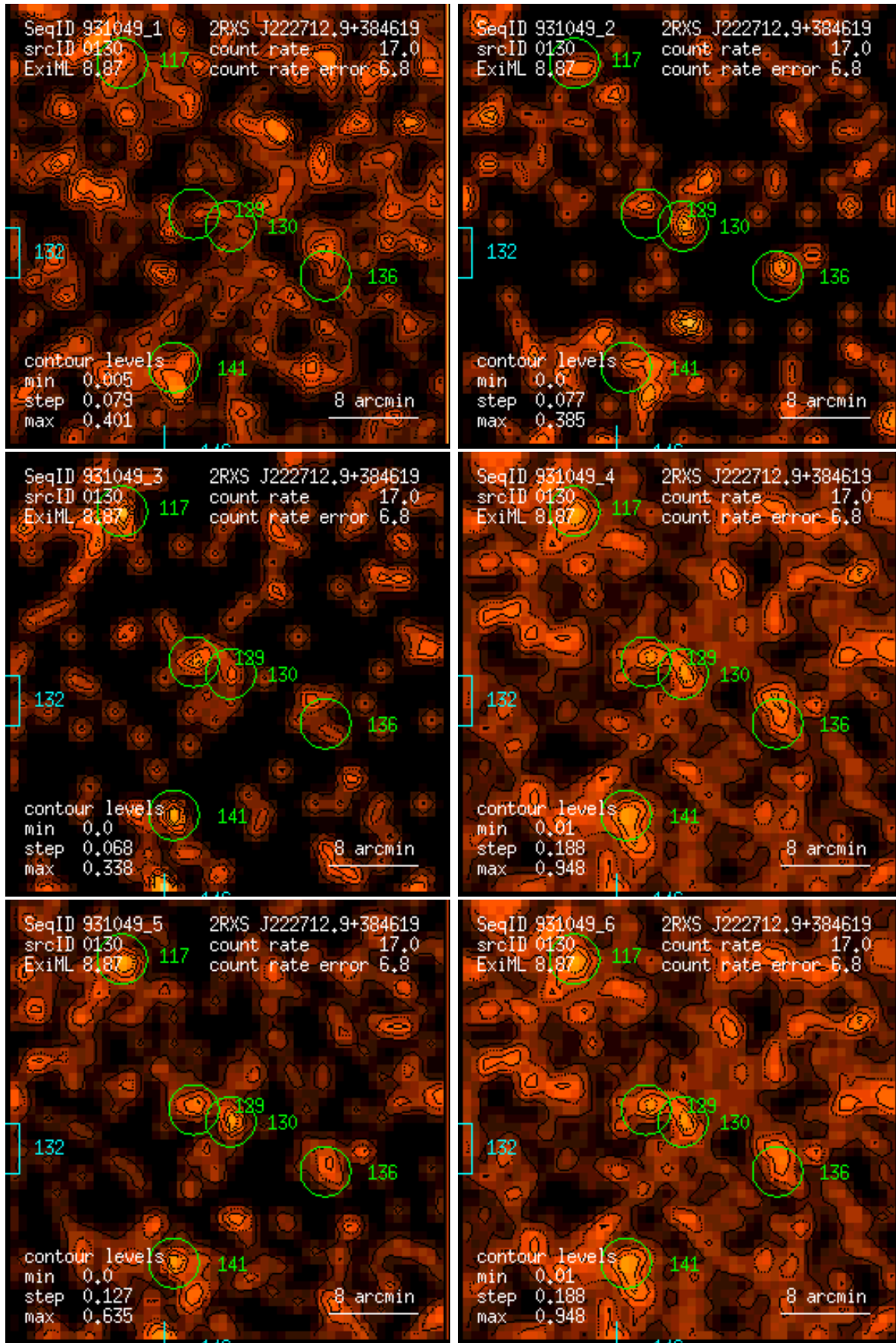
Figure 130: RASS 931049: detection 0130: band rate images, Gaussian filter: (1) PSPC channels 11 – 41, (2) 52 – 90, (3) 91 – 201, (4) 11 – 235, (5) 52 – 201, (6) 11 – 201. Broad band rates in counts/ks. Band rate contour levels in counts/ks/arcmin 2 .
