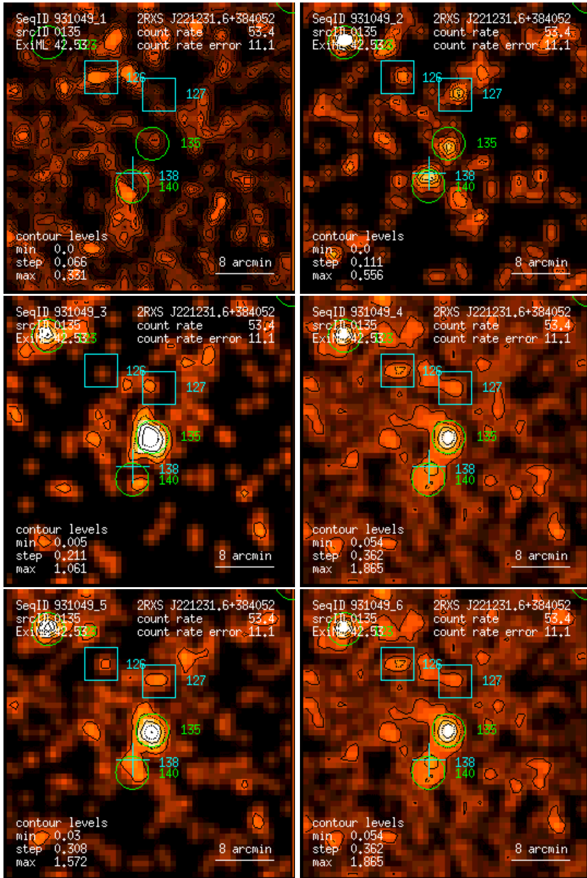
Figure 135: RASS 931049: detection 0135: band rate images, Gaussian filter: (1) PSPC channels 11 – 41, (2) 52 – 90, (3) 91 – 201, (4) 11 – 235, (5) 52 – 201, (6) 11 – 201. Broad band rates in counts/ks. Band rate contour levels in counts/ks/arcmin 2 .
