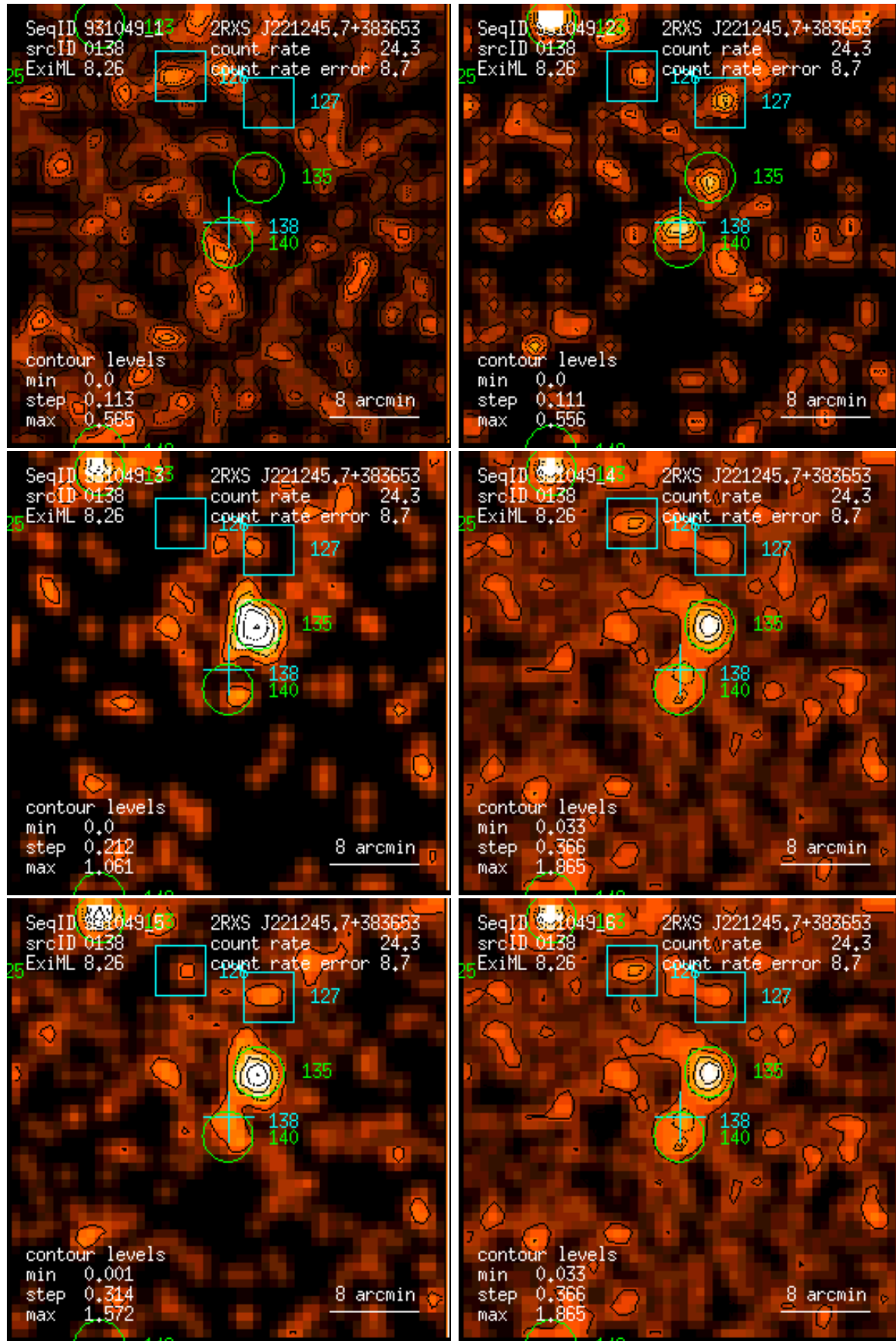
Figure 138: RASS 931049: detection 0138: band rate images, Gaussian filter: (1) PSPC channels 11 – 41, (2) 52 – 90, (3) 91 – 201, (4) 11 – 235, (5) 52 – 201, (6) 11 – 201. Broad band rates in counts/ks. Band rate contour levels in counts/ks/arcmin 2 .
