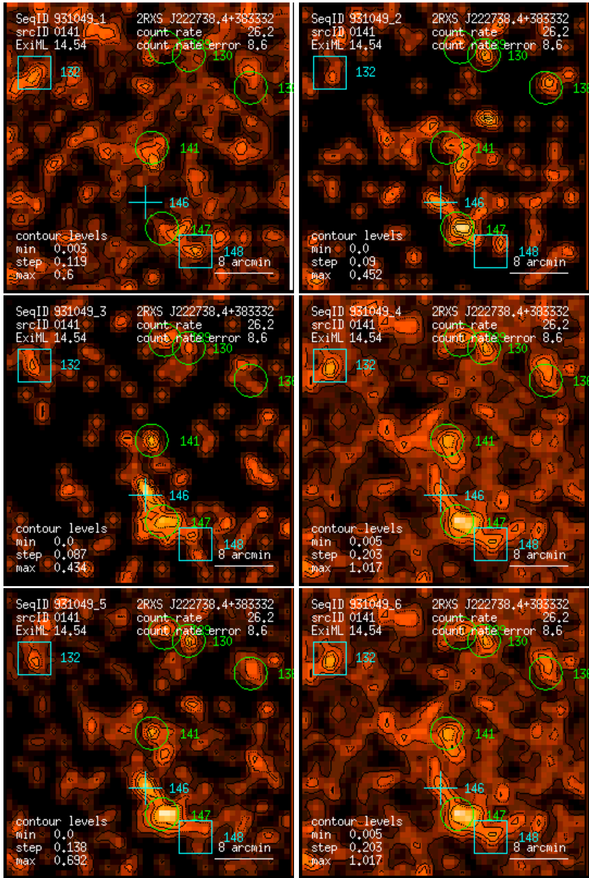
Figure 141: RASS 931049: detection 0141: band rate images, Gaussian filter: (1) PSPC channels 11 – 41, (2) 52 – 90, (3) 91 – 201, (4) 11 – 235, (5) 52 – 201, (6) 11 – 201. Broad band rates in counts/ks. Band rate contour levels in counts/ks/arcmin 2 .
