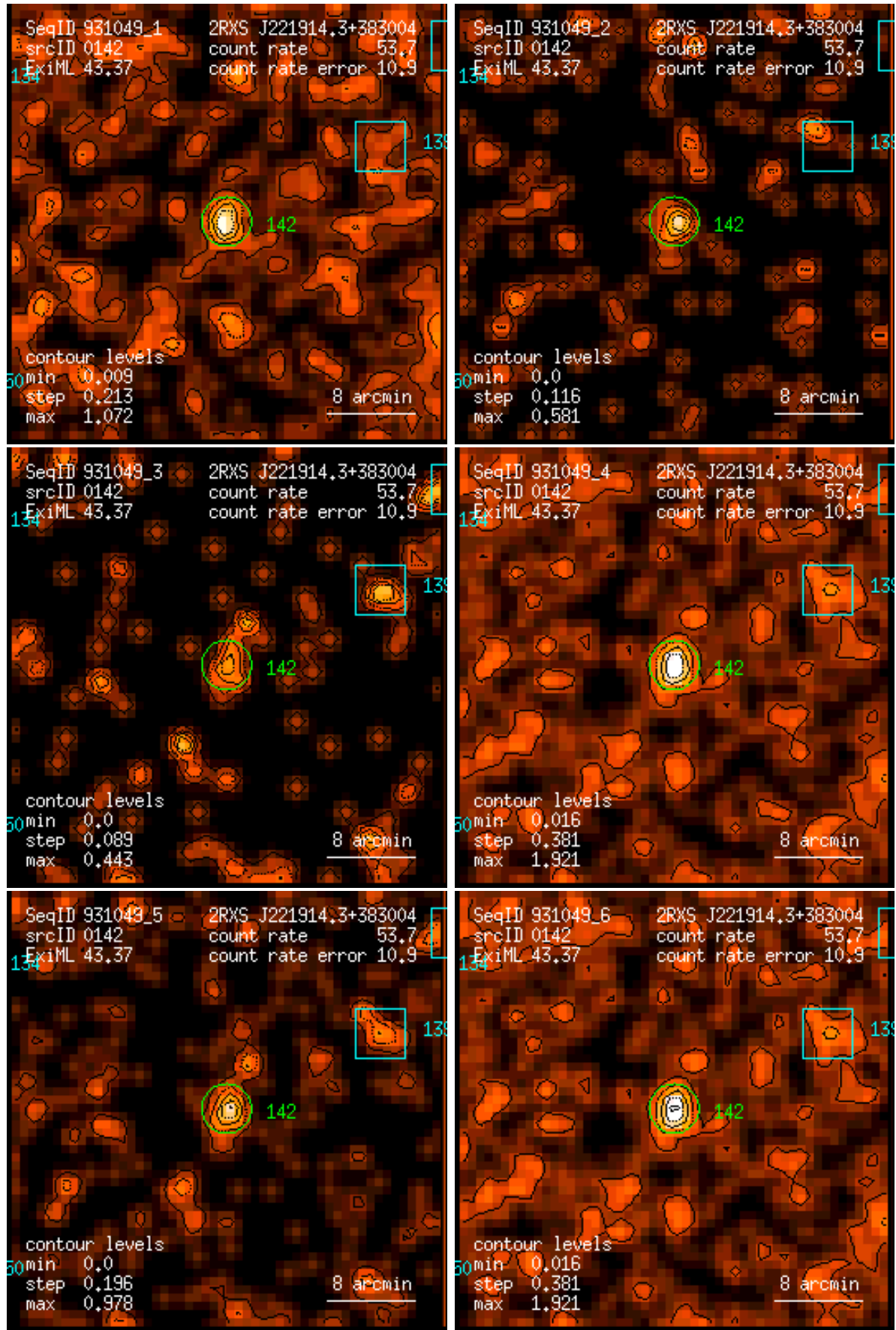
Figure 142: RASS 931049: detection 0142: band rate images, Gaussian filter: (1) PSPC channels 11 – 41, (2) 52 – 90, (3) 91 – 201, (4) 11 – 235, (5) 52 – 201, (6) 11 – 201. Broad band rates in counts/ks. Band rate contour levels in counts/ks/arcmin 2 .
