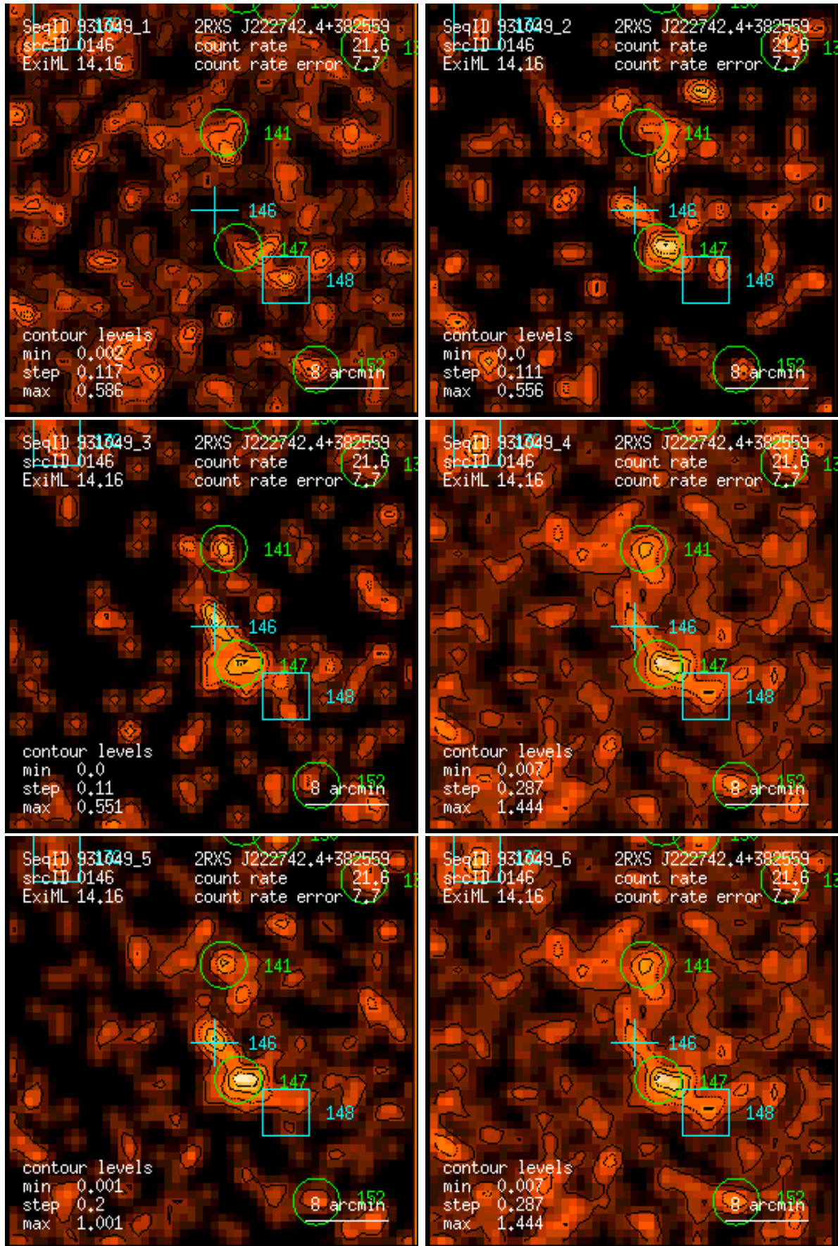
Figure 146: RASS 931049: detection 0146: band rate images, Gaussian filter: (1) PSPC channels 11 – 41, (2) 52 – 90, (3) 91 – 201, (4) 11 – 235, (5) 52 – 201, (6) 11 – 201. Broad band rates in counts/ks. Band rate contour levels in counts/ks/arcmin 2 .
