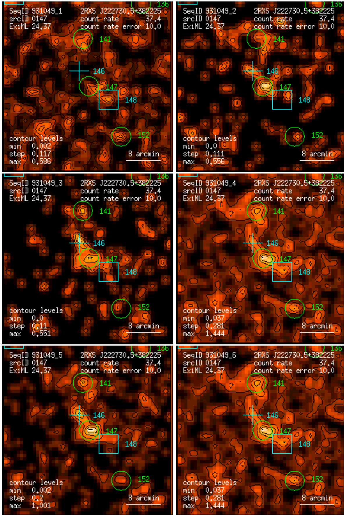
Figure 147: RASS 931049: detection 0147: band rate images, Gaussian filter: (1) PSPC channels 11 – 41, (2) 52 – 90, (3) 91 – 201, (4) 11 – 235, (5) 52 – 201, (6) 11 – 201. Broad band rates in counts/ks. Band rate contour levels in counts/ks/arcmin 2 .
