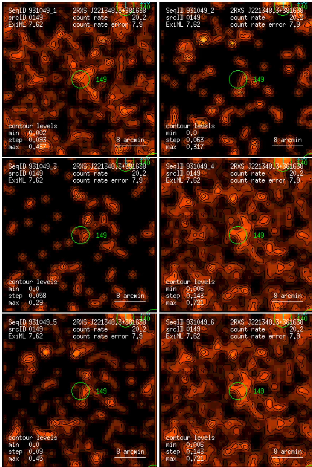
Figure 149: RASS 931049: detection 0149: band rate images, Gaussian filter: (1) PSPC channels 11 – 41, (2) 52 – 90, (3) 91 – 201, (4) 11 – 235, (5) 52 – 201, (6) 11 – 201. Broad band rates in counts/ks. Band rate contour levels in counts/ks/arcmin 2 .
