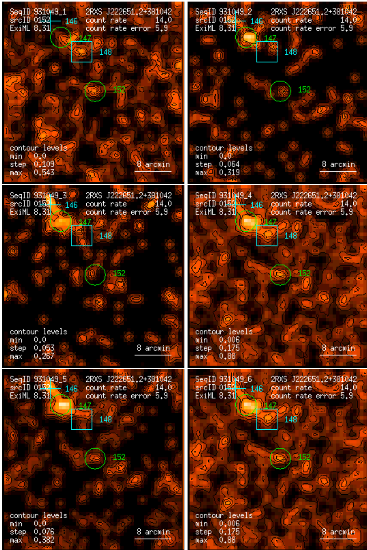
Figure 152: RASS 931049: detection 0152: band rate images, Gaussian filter: (1) PSPC channels 11 – 41, (2) 52 – 90, (3) 91 – 201, (4) 11 – 235, (5) 52 – 201, (6) 11 – 201. Broad band rates in counts/ks. Band rate contour levels in counts/ks/arcmin 2 .
