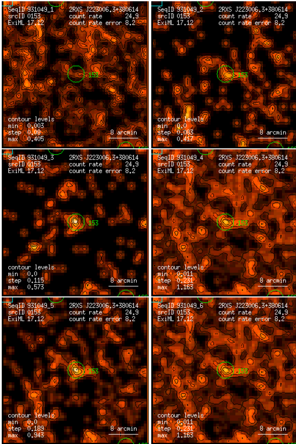
Figure 153: RASS 931049: detection 0153: band rate images, Gaussian filter: (1) PSPC channels 11 – 41, (2) 52 – 90, (3) 91 – 201, (4) 11 – 235, (5) 52 – 201, (6) 11 – 201. Broad band rates in counts/ks. Band rate contour levels in counts/ks/arcmin 2 .
