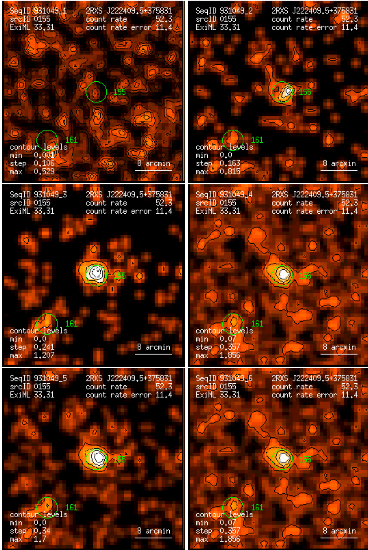
Figure 155: RASS 931049: detection 0155: band rate images, Gaussian filter: (1) PSPC channels 11 – 41, (2) 52 – 90, (3) 91 – 201, (4) 11 – 235, (5) 52 – 201, (6) 11 – 201. Broad band rates in counts/ks. Band rate contour levels in counts/ks/arcmin 2 .
