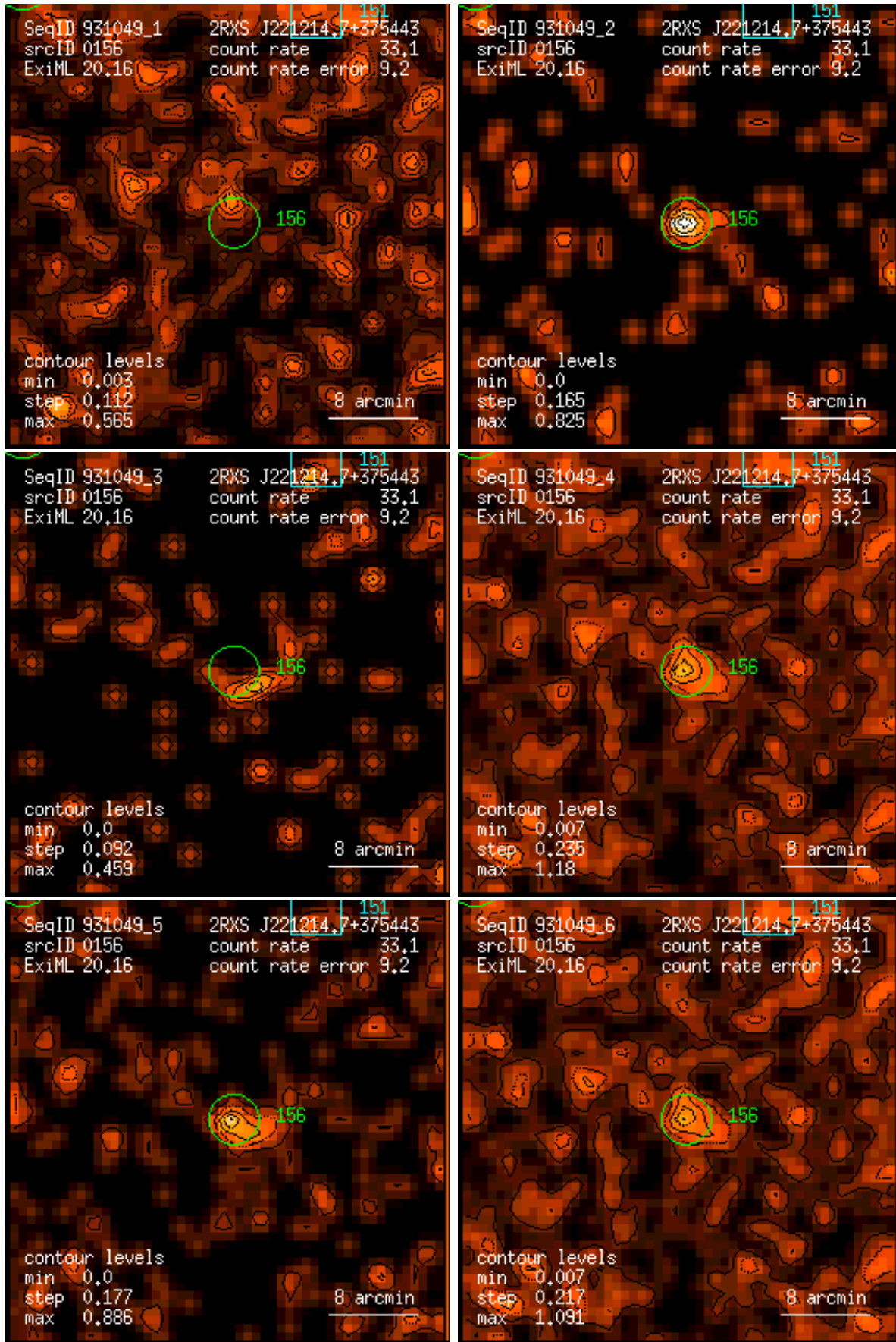
Figure 156: RASS 931049: detection 0156: band rate images, Gaussian filter: (1) PSPC channels 11 – 41, (2) 52 – 90, (3) 91 – 201, (4) 11 – 235, (5) 52 – 201, (6) 11 – 201. Broad band rates in counts/ks. Band rate contour levels in counts/ks/arcmin 2 .
